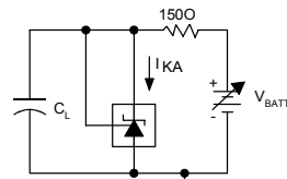
TEST CIRCUIT FOR CURVE A
