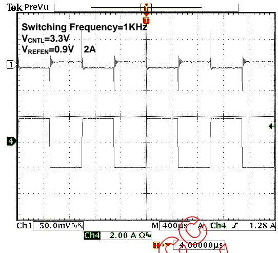
Figure 13. 0.9V OUT @ 2A Transient Response
