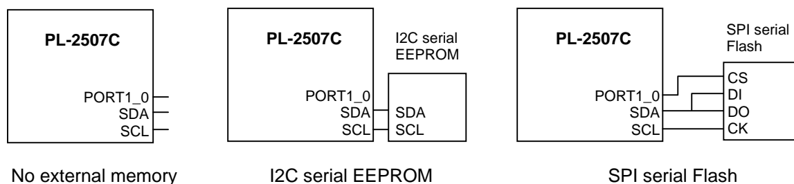
Figure 5-1 External Serial Memory Implementation
