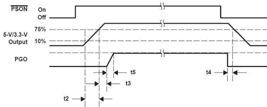
Figure 1. Timing of \overline{\text{PSON}} and PGO
