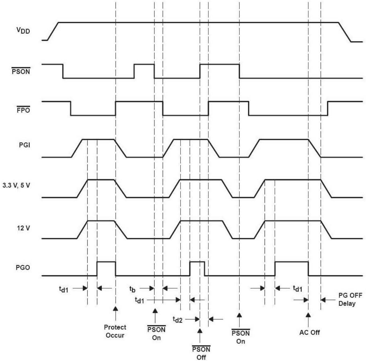
timing diagram
