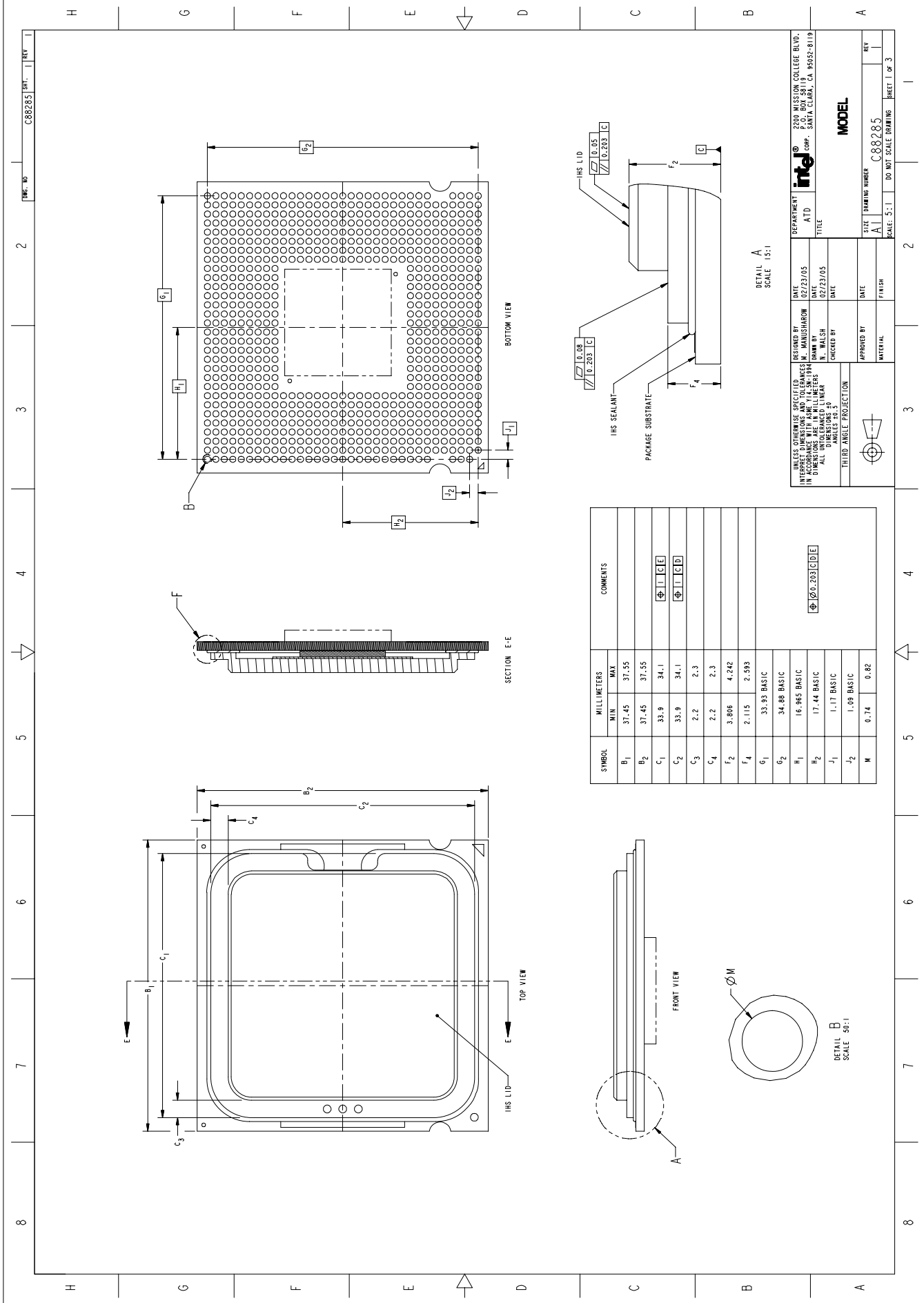
Figure 8. Processor Package Drawing Sheet 1 of 3
