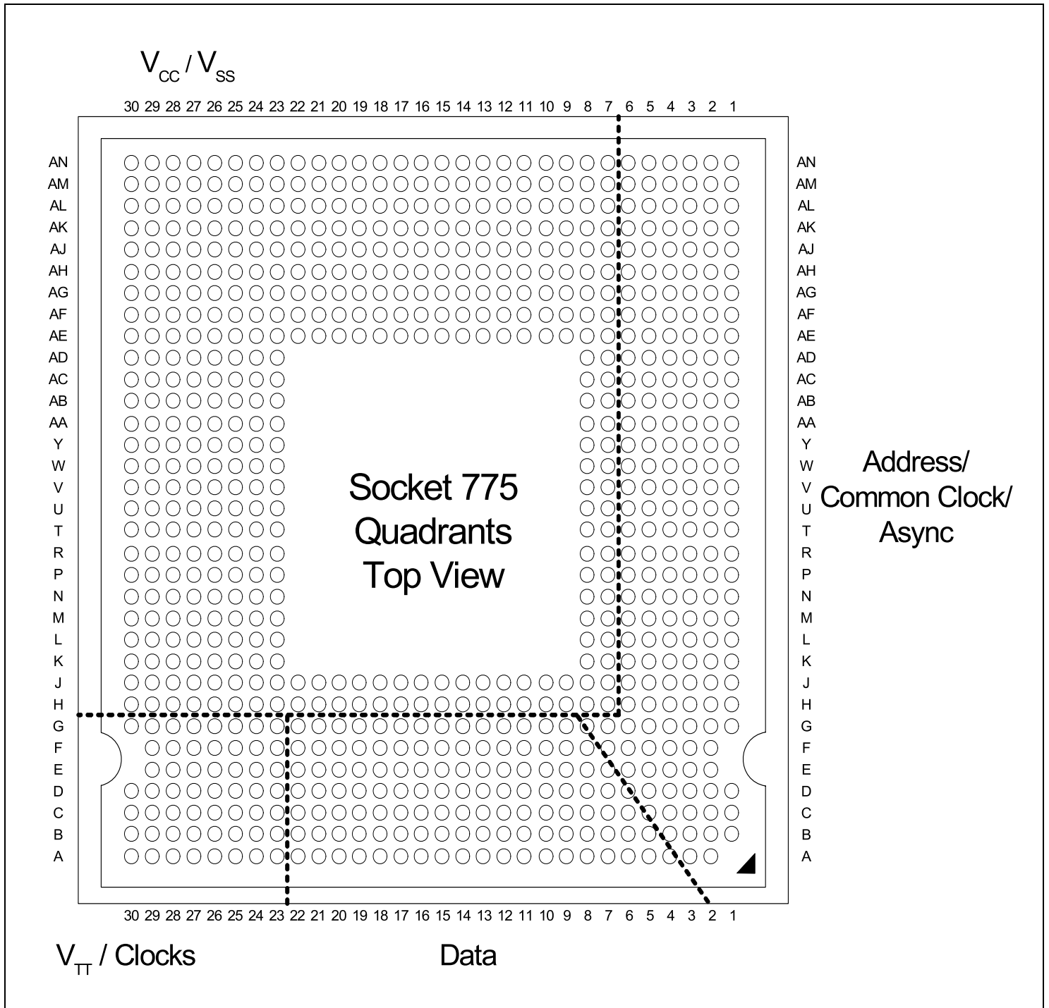
Figure 16. Processor Land Coordinates and Quadrants (Top View)
